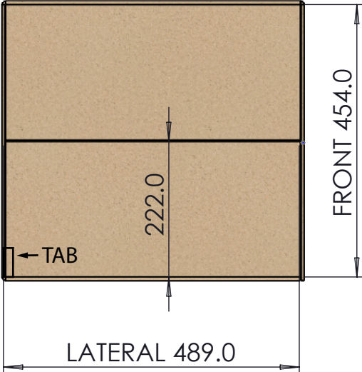
UPPER VIEW (INTERNAL DIMENSIONS)
