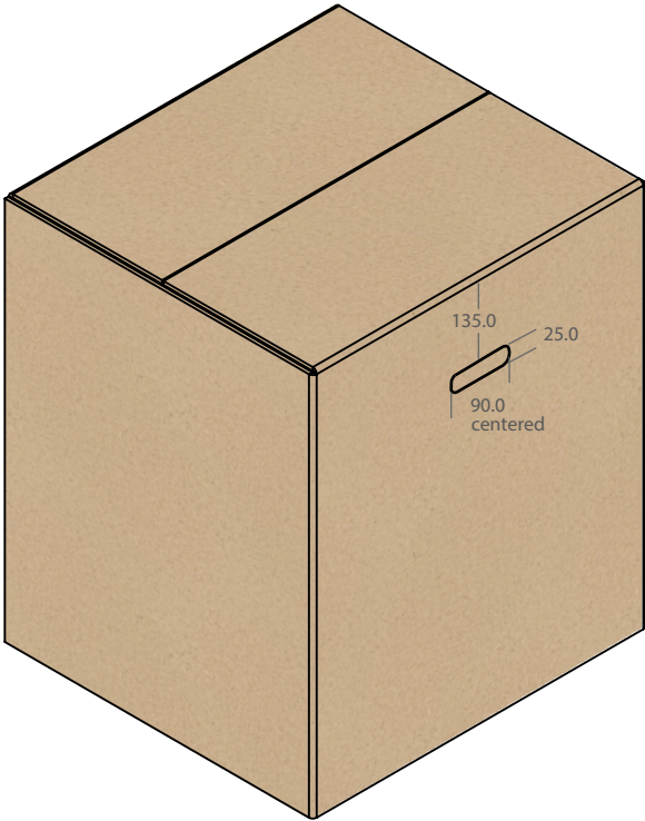
ISOMETRIC VIEW (INTERNAL DIMENSIONS)
