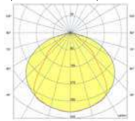
Systeo SLIM Clear + optics 90°
