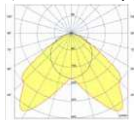
Systeo SLIM Clear + batwing optics
