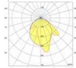
Systeo SLIM Clear + wallwasher optics
