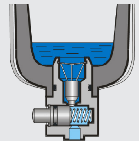
Purga manual
