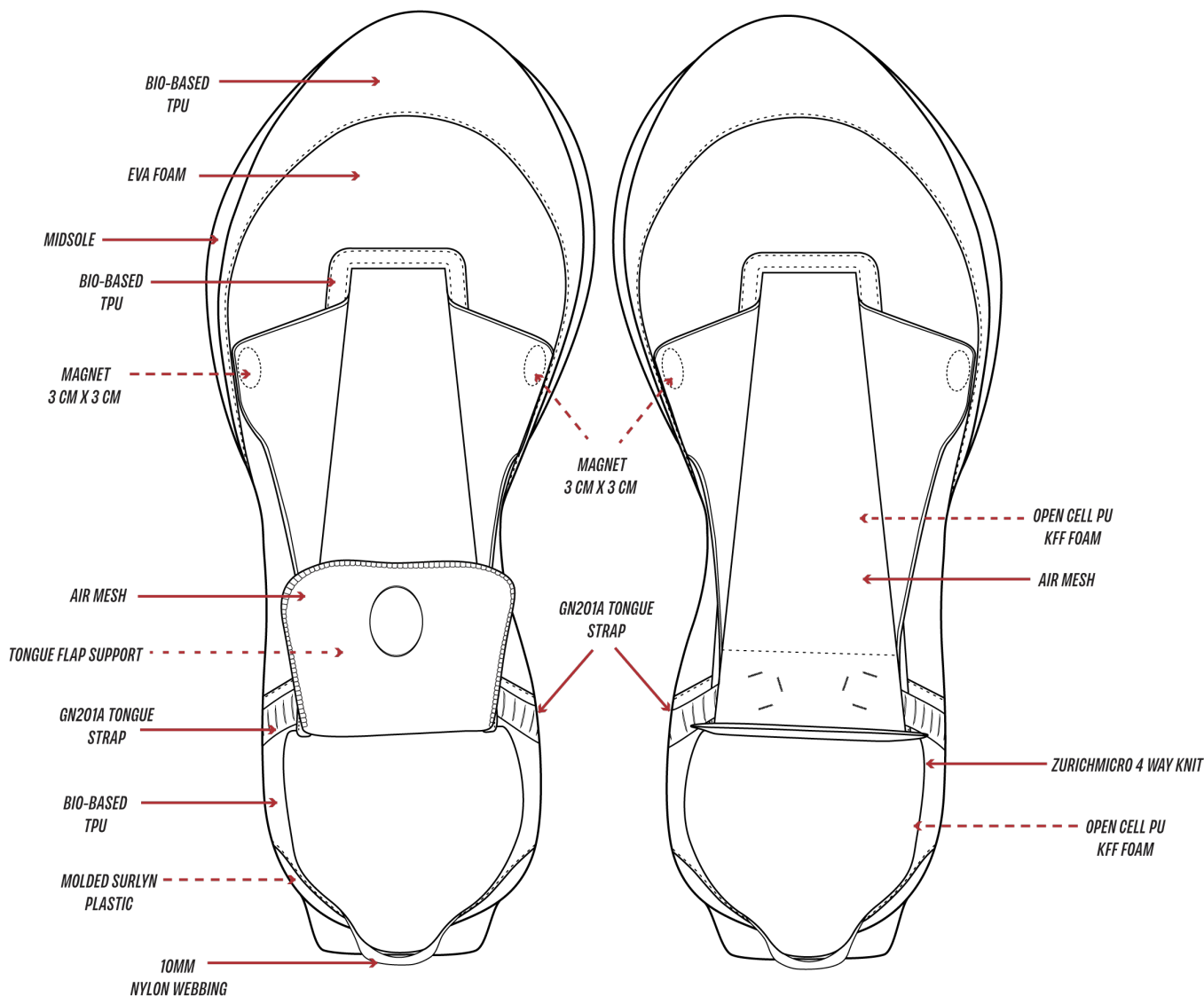
TOP VIEW - MATERIAL CALLOUTS
