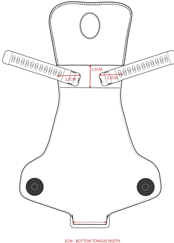
SHOWING HOW TONGUE STRAPS ARE SEWN IN - VIEWING FROM UNDER THE TONGUE'S BACKSIDE COVER FABRIC
