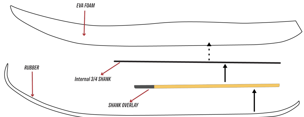
LATERAL EXPLODED VIEW
