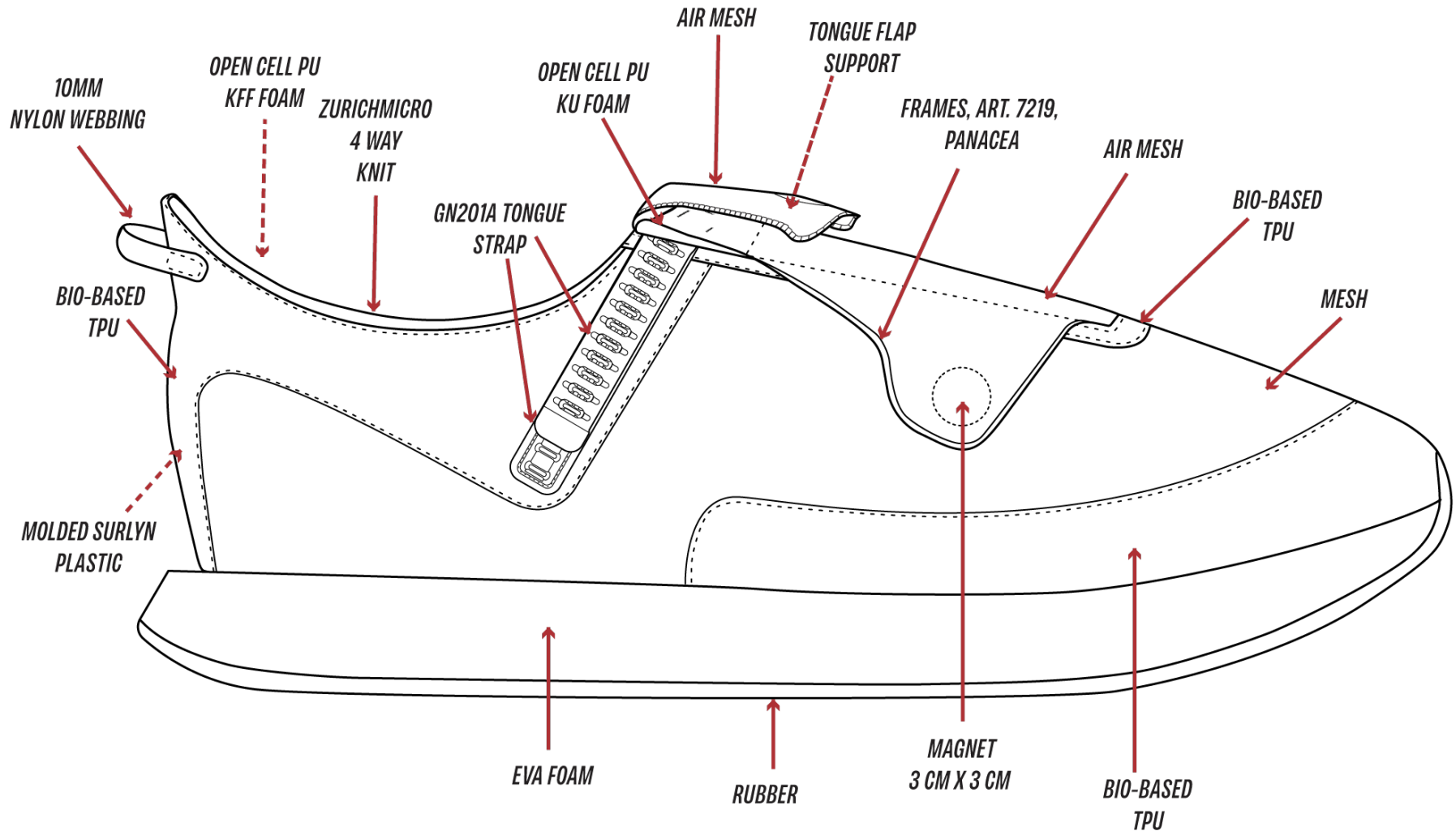
MEDIAL VIEW (TONGUE FOLDED/STRAP DOWN) MATERIAL CALLOUTS
