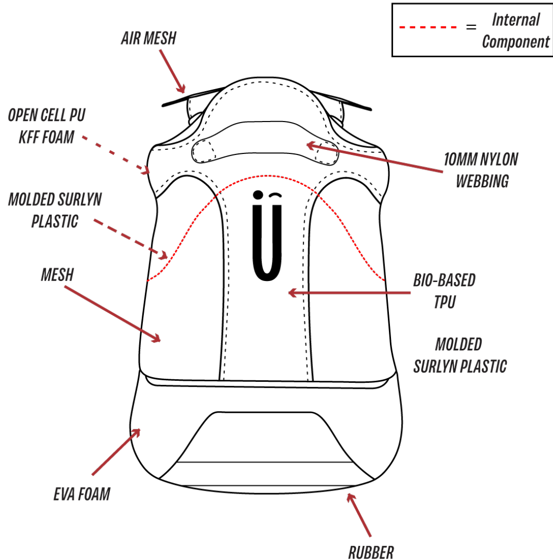
HEEL VIEW MATERIAL CALLOUTS
