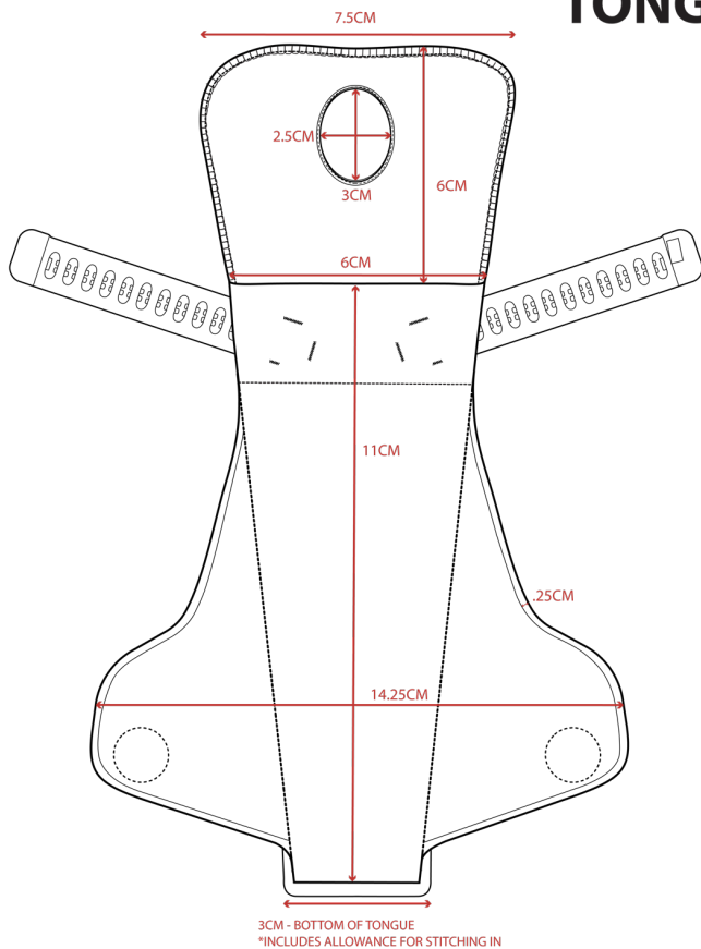
COVER FABRIC ON BACK OF TONGUE - COVERING THE SEW IN POINTS OF TOP AND BOTTOM TONGUE STRAPS
