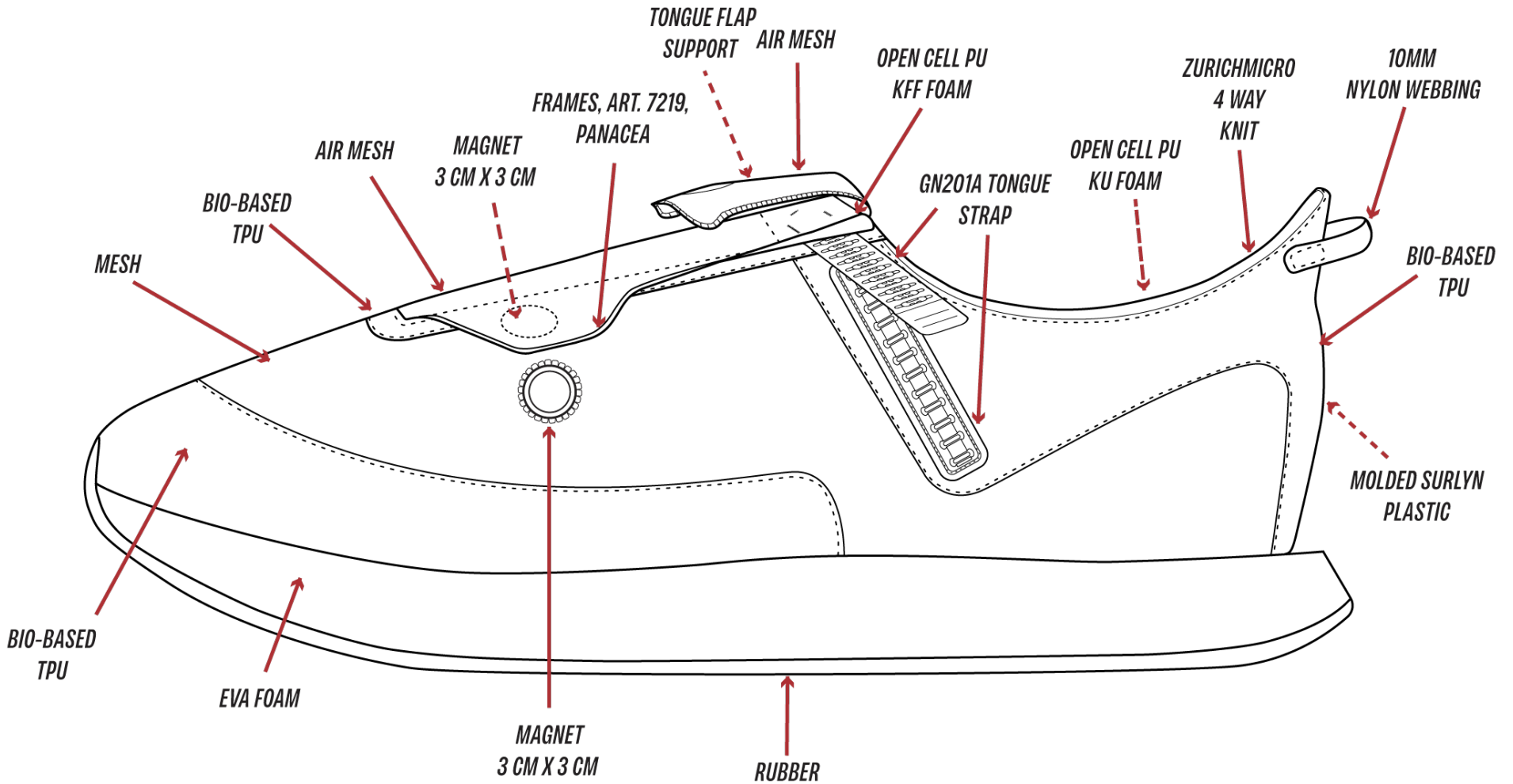
LATERAL VIEW (TONGUE FOLDED/STRAP UP) MATERIAL CALLOUTS
