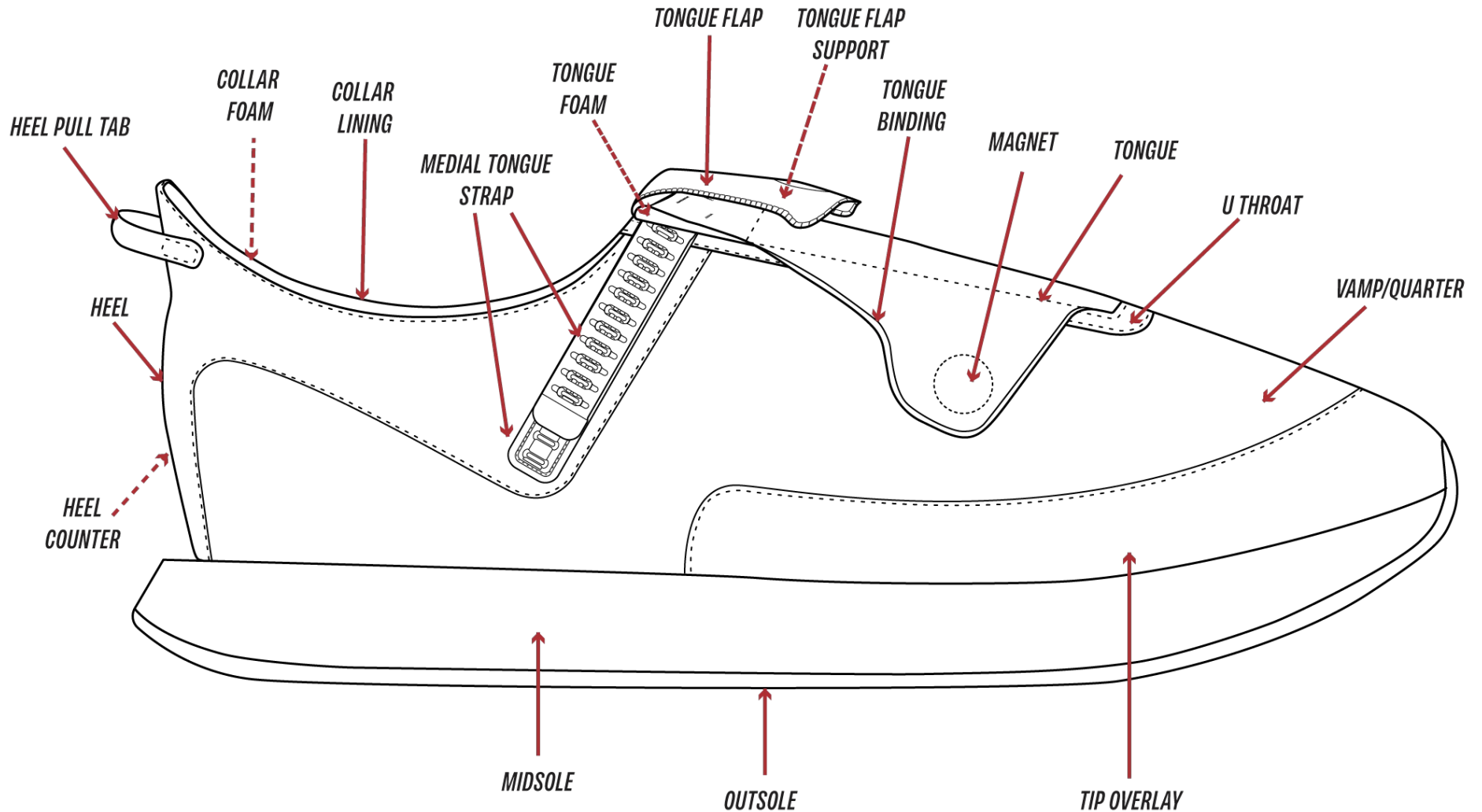
MEDIAL VIEW (TONGUE FOLDED/STRAP DOWN) COMPONENT CALLOUTS
