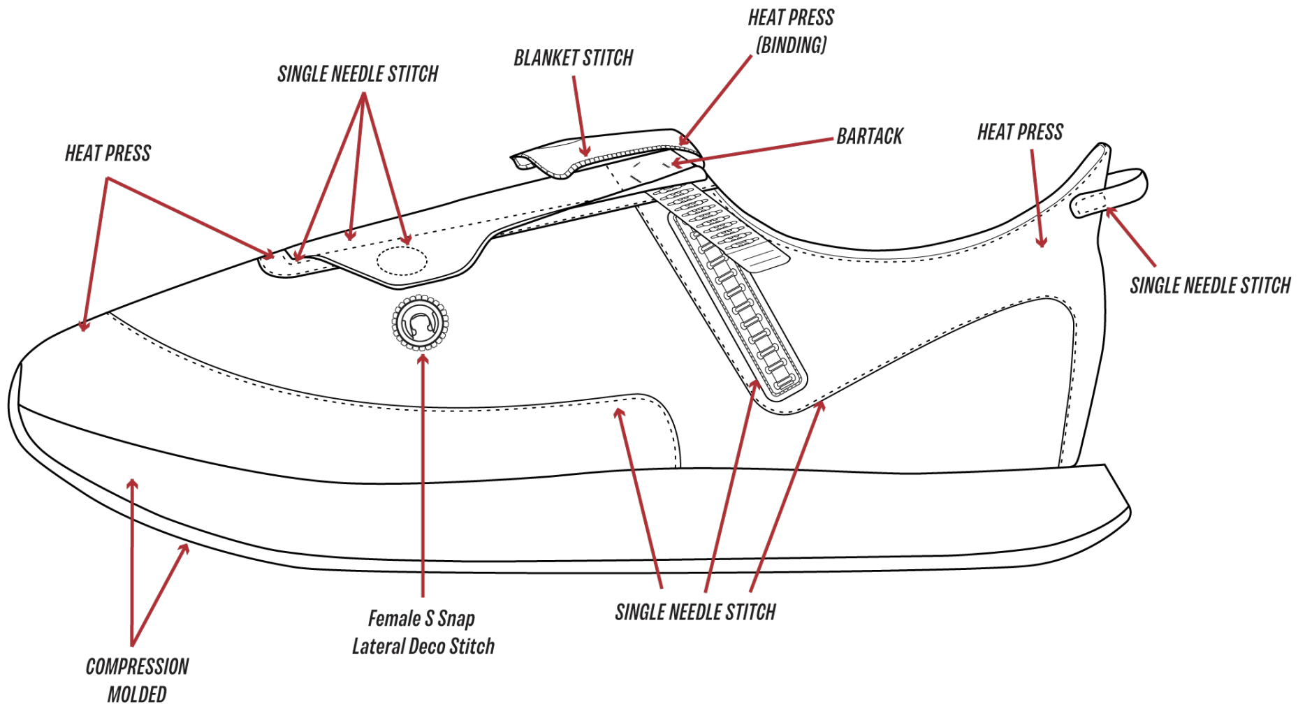
LATERAL VIEW (TONGUE FOLDED/STRAP UP) CONSTRUCTION CALLOUTS
