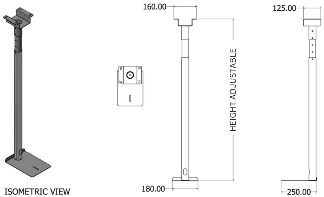
Camera Ceiling Mount Model - VT-CCM
