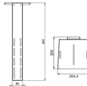
Camera Ledge
