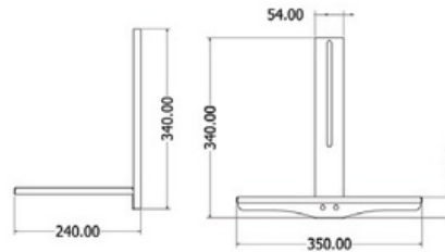
Equipment Tray : ET-LGFS-6598
