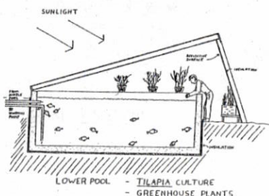
Fig. 13 Greenhouse - Fish Culture Structure
