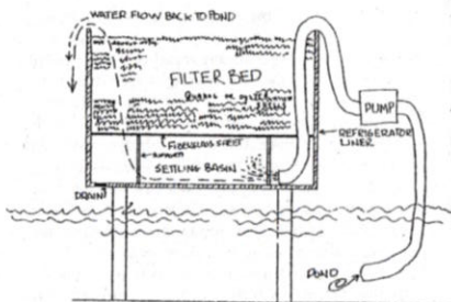
Fig. 5 - Filter
