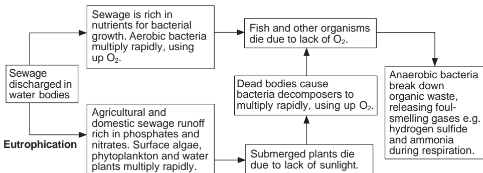
Water pollution and eutrophication
