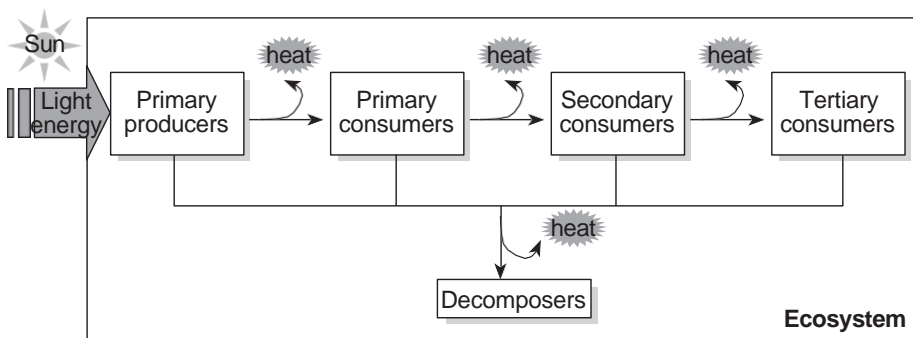
Flow of energy through an ecosystem
