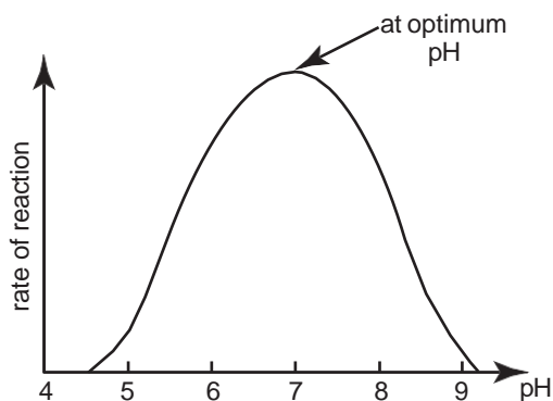
Effect of pH on the rate of reaction of amylase
