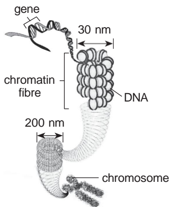
Folding of DNA
