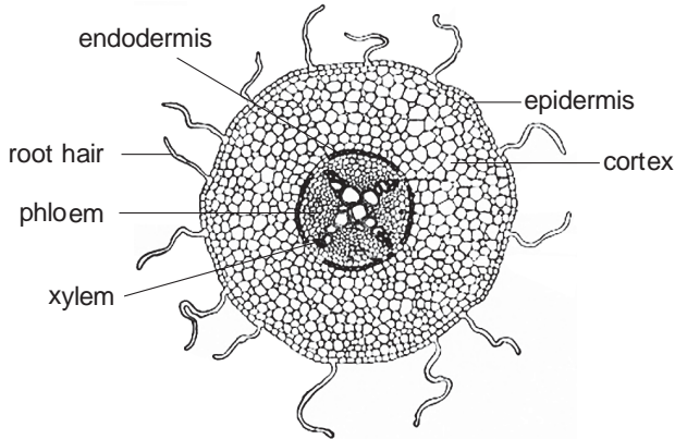
Transverse section of a root
