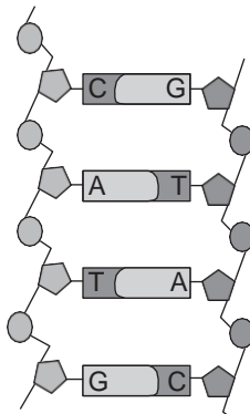
Complementary base pairing
