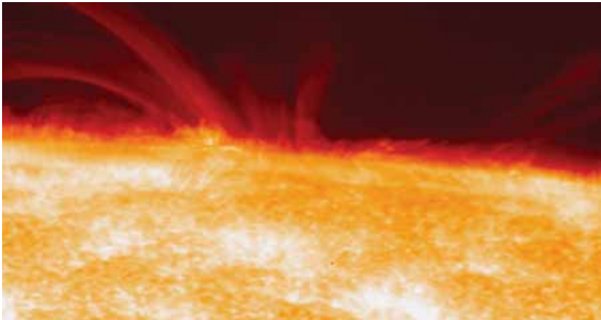
This picture was taken by Hinode's Solar Optical Telescope on November 11, 2006. In the foreground, this image reveals the fine-scale structure in the chromosphere that extends outward above the top of the convection cells, or granulation, of the visible solar surface layer, the photosphere. In the background, plasma above a sunspot traces out magnetic field lines into the corona.
