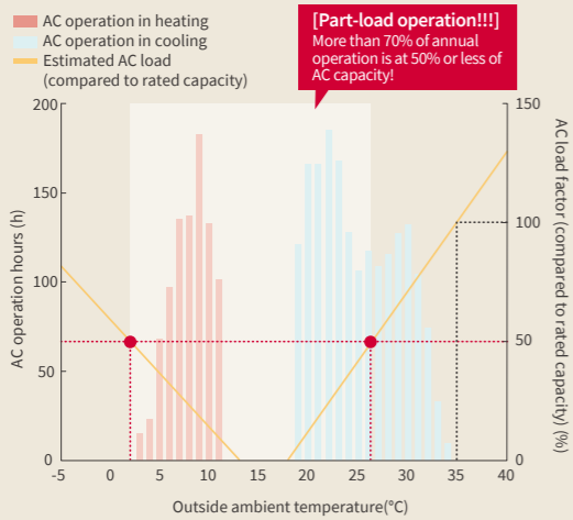
AC operating hours per outside ambient temperature in Office (Japan, Tokyo) (concerning Large Split & VRF) *1
