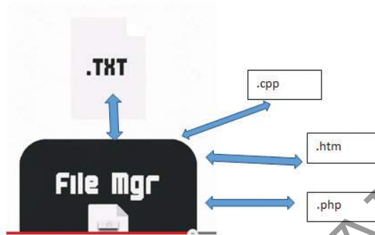
Figure 5.8 - File Management
