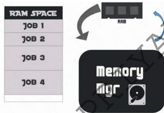
Figure 5.6 - Memory Management
