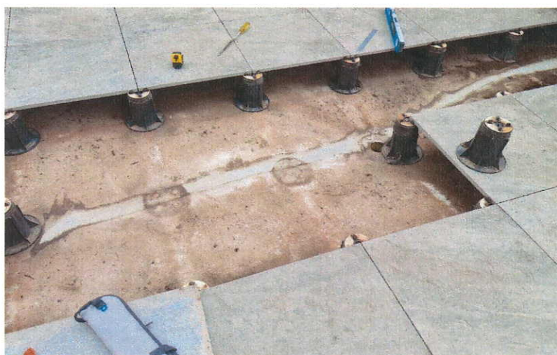
PHOTOGRAPH 7 shows dirt and debris accumulated on the waterproofing membrane beneath the tiles after approximately 2 years. In this image, the dirt was cleaned off the membrane to examine a failure in the membrane beneath
