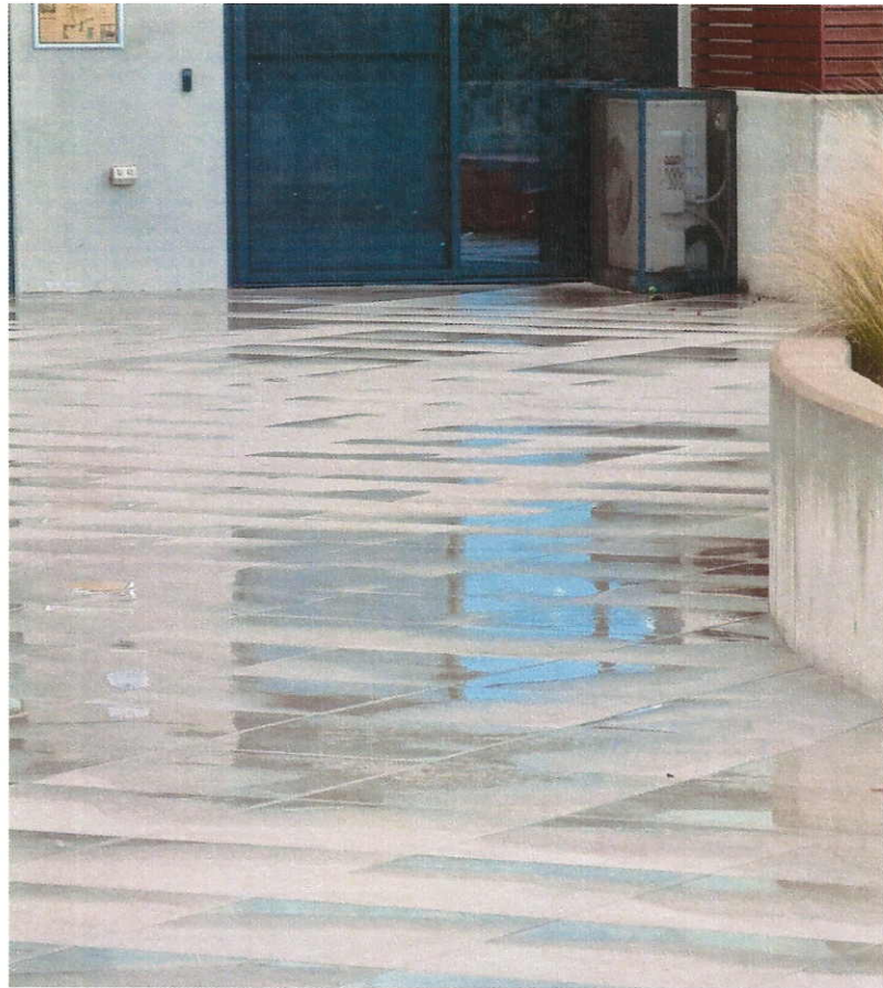
PHOTOGRAPH 5 depicts water retention on a podium tile installation during the morning at 10 am after a night of rain
