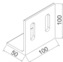
角码 50+100x100x8
