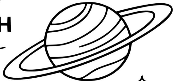
SATURN
