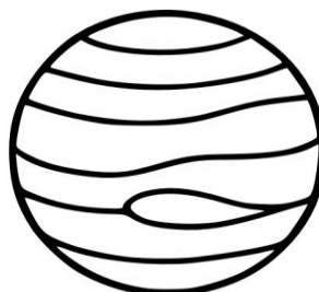
NEPTUNE
