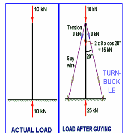
Fig. 14. Post compression
