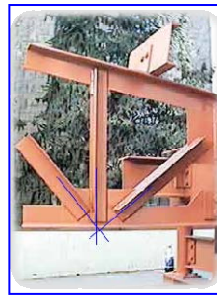
Fig. 9. Truss connections
