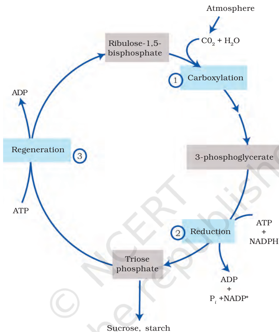
Figure 11.8 The Calvin cycle proceeds in three stages : (1) carboxylation, during which CO 2 combines with ribulose-1,5-bisphosphate; (2) reduction, during which carbohydrate is formed at the expense of the photochemically made ATP and NADPH; and (3) regeneration during which the CO 2 acceptor ribulose-1,5-bisphosphate is formed again so that the cycle continues
