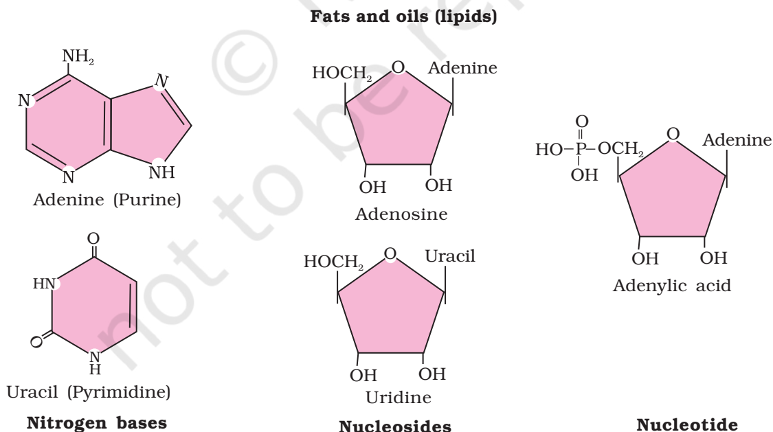
Figure 9.1 Diagrammatic representation of small molecular weight organic compounds in living tissues
