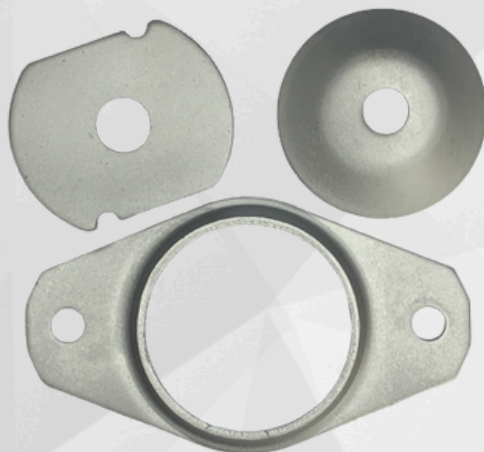
IA 001 (Flange)
