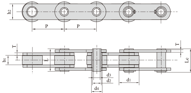
with F flanged rollers type
