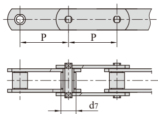
5.Welded pins with plates
