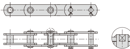
5.Welded pins with plates
