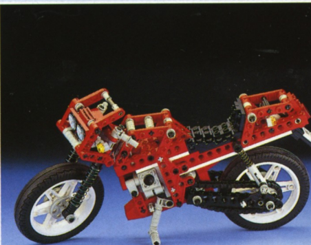
8422 LEGO TECHNIC V-Twin Super Bike with suspension on both wheels and a chain driven, two cylinder engine. Includes building instructions for a Dragster. Can be motorised with set 8720. From 9 years.
