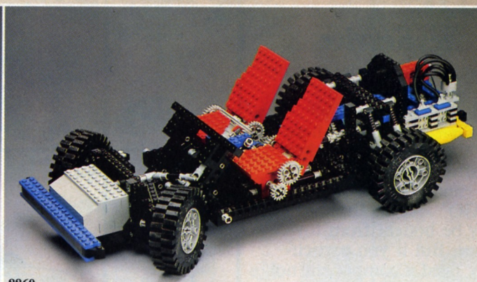
8860 Car chassis. With steering, adjustable seats, suspension, 4 cylinder box engine with fan, and differential gear. Building instructions for 3 models. Around £ 45.00
