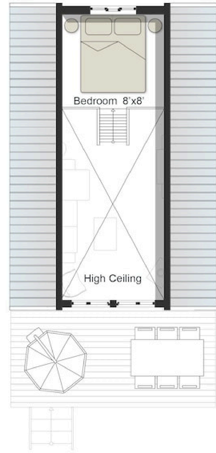
Mezzanine Floor Plan
