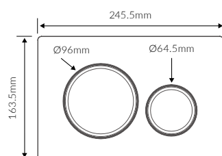
ROUND FLUSH PLATE
