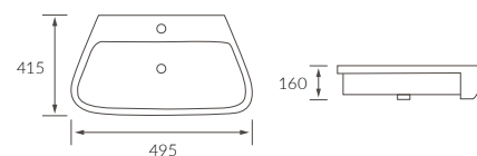
SEMI RECESSED BASIN 495 x 415mm
