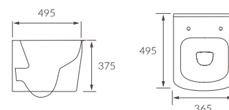
WALL HUNG PAN
