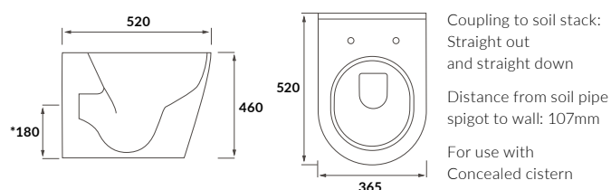
RIMLESS BACK TO WALL PAN COMFORT HEIGHT
