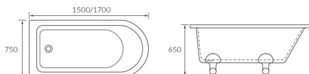
BANDA FLOORSTANDING BATH
