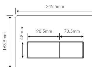
RECTANGLE FLUSH PLATE
