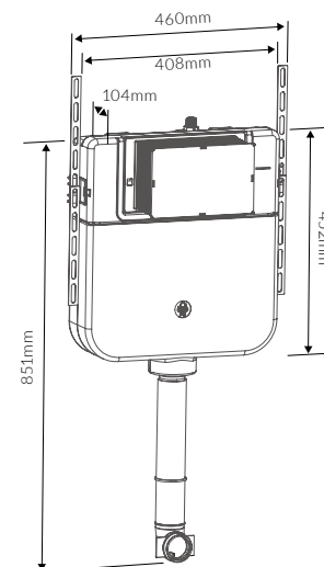
SLIM CONCEALED CISTERN
