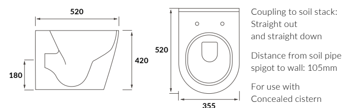
BACK TO WALL PAN
