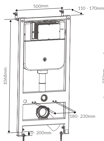
WALL HUNG WC FRAME Incl. Cistern
