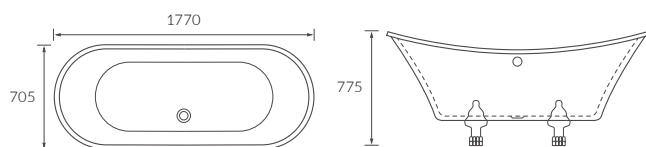
BISCAY FLOORSTANDING BATH
