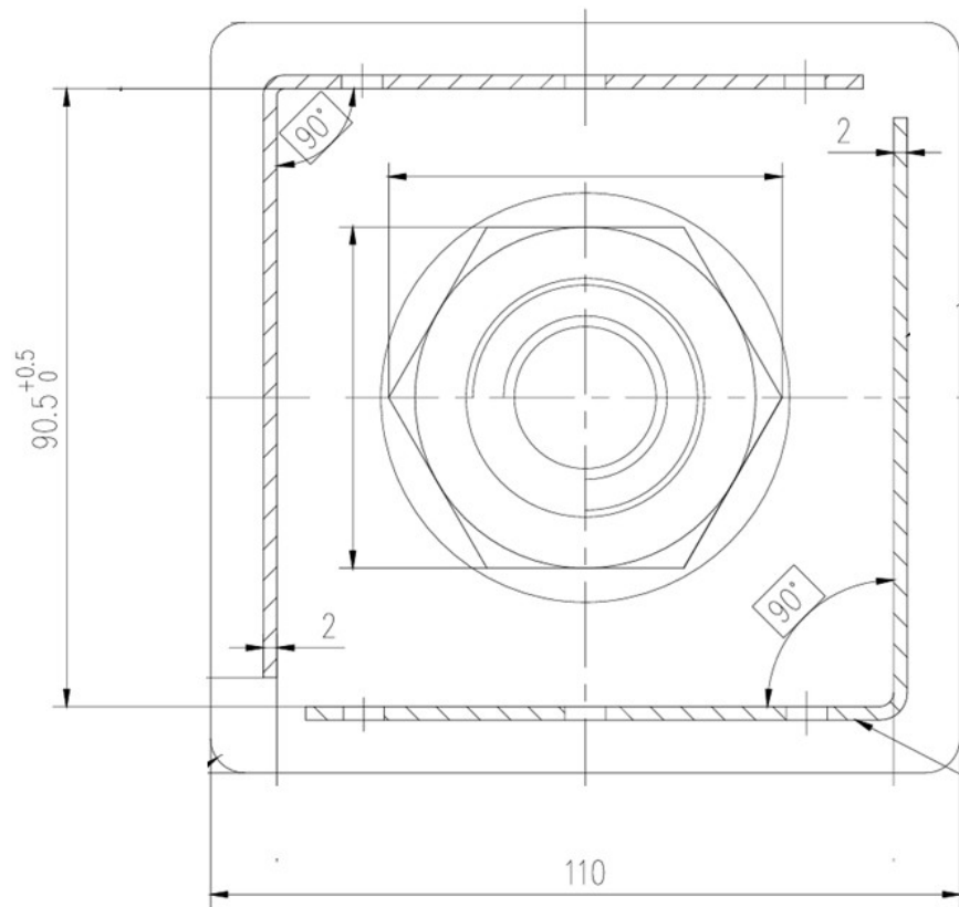
90mm House Stump Top
