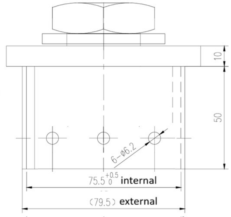
75mm House Stump Top
