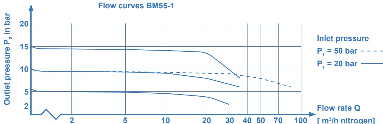
Flow curves BM55-1
