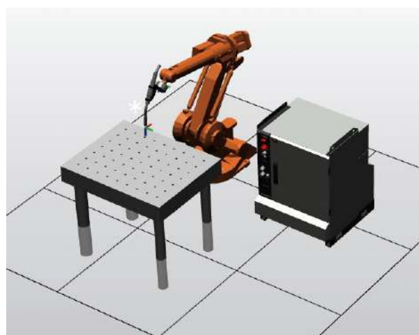
DLRB-1410 焊接机器人实训系统 Welding Robot Training System
