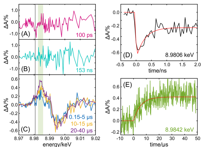
Figure 5. (A–C) X-ray transient absorption difference spectra of 3 mM CuOTf and 0.3 M cyclohexene in THF at various pump–probe delay times. (D) Short-time kinetic trace measured at the probe energy indicated by the vertical line in panels A–C. (E) Long-time kinetic trace averaged over the probe bandwidth indicated by the vertical bar in panels A–C.
