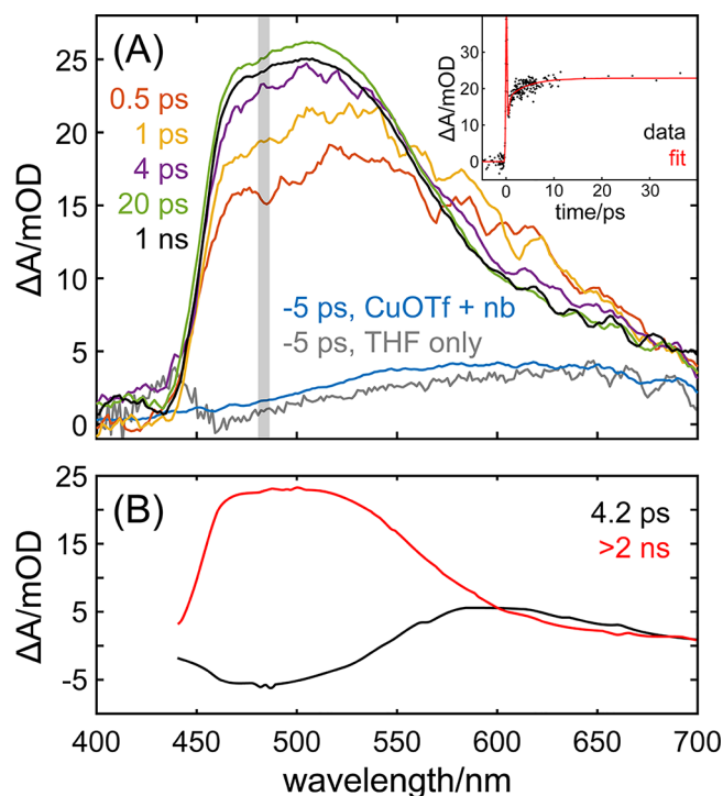
Figure 6. (A) Optical transient absorption spectra of 6 mM CuOTf and 0.6 M norbornene in THF at representative pump–probe delay times, showing the growth of the ESA signal over the first several picoseconds. The -5 ps spectra of both the Cu + nb sample in THF (blue) and neat THF (gray) show a weak ESA signal due to the multiphoton ionization of the solvent. The early time kinetic trace taken from the probe region indicated by the vertical bar is shown in the inset with the corresponding multiexponential fit. (B) Decay-associated spectra of CuOTf + nb obtained from a global fit of the optical transient absorption data.
