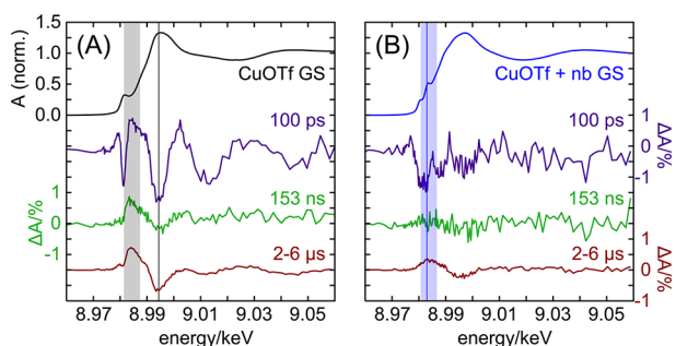
Figure 2. Ground-state (GS) and difference Cu K-edge XANES spectra of 6 mM CuOTf in THF (A) and 6 mM CuOTf and 0.6 M norbornene in THF (B) at several pump–probe delay times. The probe energies for which the short- and long-time kinetics are plotted in Figure 4 are indicated by vertical lines and bars, respectively.
