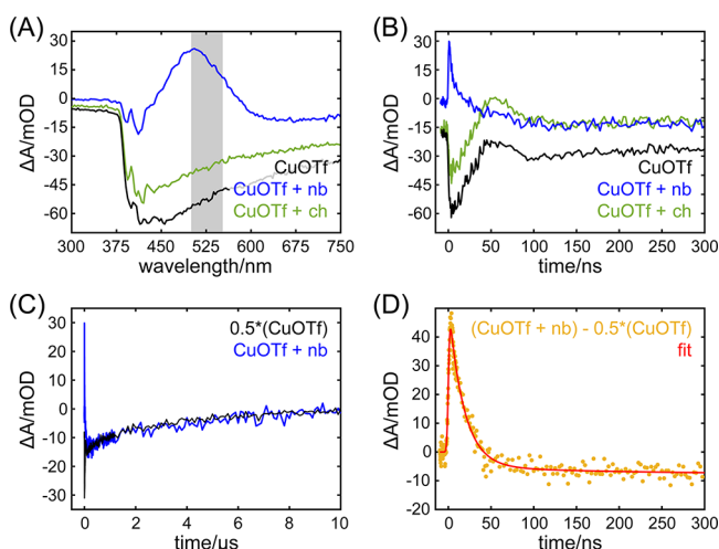
Figure 7. (A) Optical transient absorption spectra of 6 mM CuOTf in THF (black), 6 mM CuOTf and 0.6 M norbornene in THF (blue), and 6 mM CuOTf and 0.6 M cyclohexene in THF (green) averaged over a pump–probe delay window of 2.8 to 3.8 ns. (B) Kinetic traces obtained by averaging over the probe window indicated by the vertical bar in panel A. (C) Long-time kinetic traces of CuOTf alone scaled by a factor of 0.5 and CuOTf + nb, highlighting the identical kinetics observed on the microsecond time scale for the different samples. (D) Kinetic trace of CuOTf + nb with the contributions from multiphoton solvent ionization subtracted (mustard) and the corresponding fit (red) to a single-exponential decay and a persistent offset.
