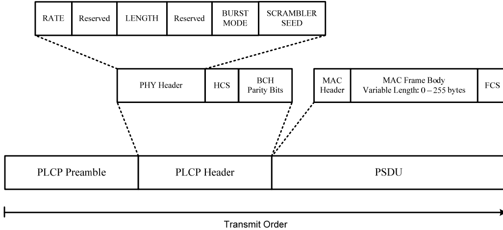
Figure 116 —Standard PPDU structure
