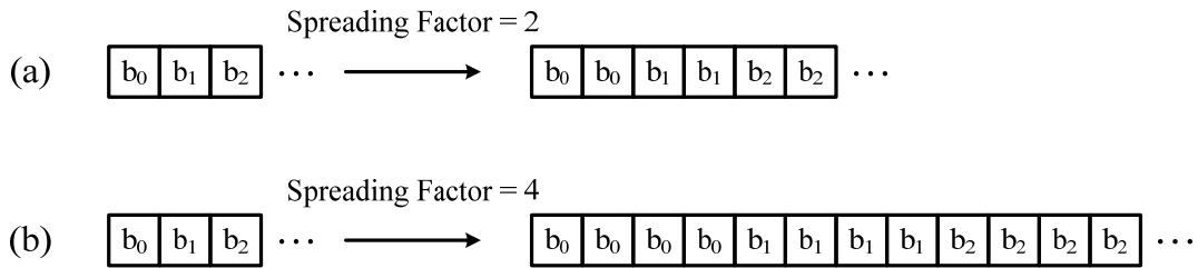
Figure 123—Spreading scheme
