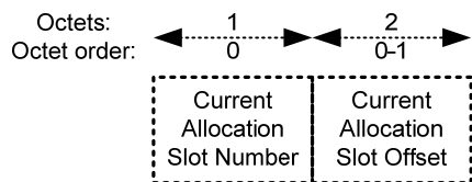
Figure 37—Frame Payload format for I-Ack frames
