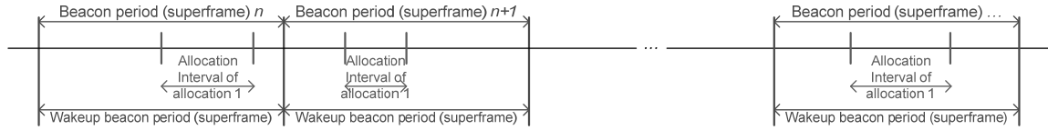
(a3) Shifted and reduced/expanded 1-periodic allocation in beacon or non-beacon mode with superframes
