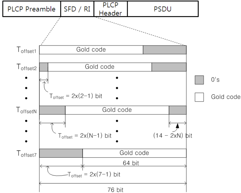
Figure 164 —Zero padding method for RI signal generation
