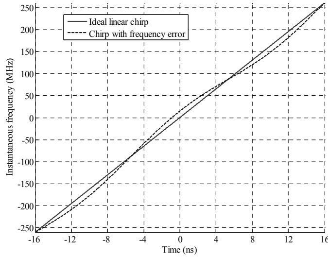
Figure 147 —Example of an instantaneous frequency function for T_w = 32 ns
