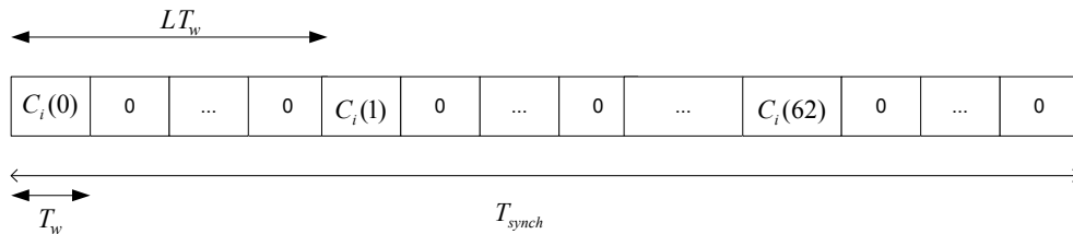
Figure 136 —Construction of synchronization symbols from a Kasami sequence
