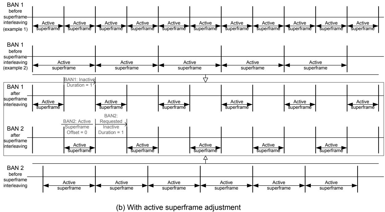
Figure 101 —Active superframe interleaving illustration
