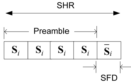
Figure 143—Structure of SHR with DBPSK modulation
