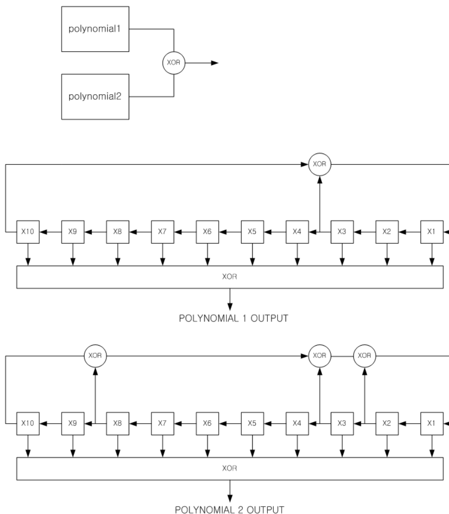
Figure 162 —Gold code generator
