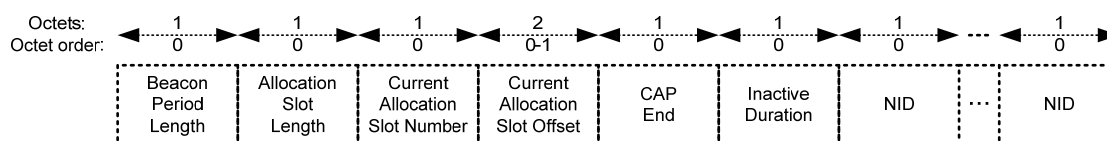
Figure 41—Frame Payload format for B2 frames
