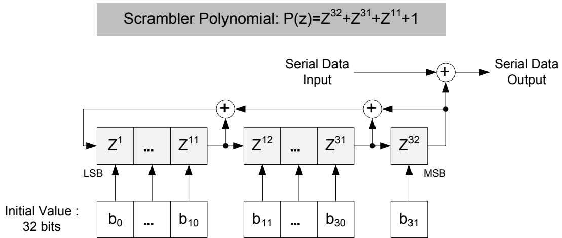
Figure 167 —Block diagram of scrambler
