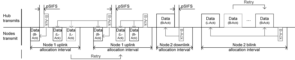
Figure 63—Late acknowledgement (L-ACK) and block acknowledgement (B-Ack) illustration
