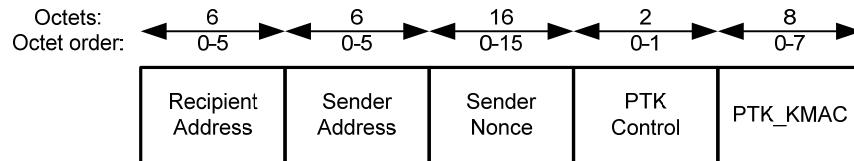
Figure 23—Frame Payload format for PTK frames
