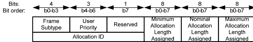
Figure 54—Type-II Unscheduled Allocation Assignment format
