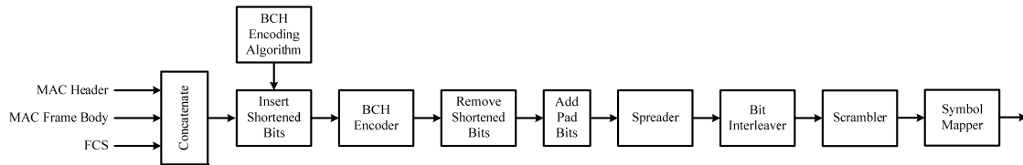
Figure 121 —Block diagram of PSDU construction for transmission
