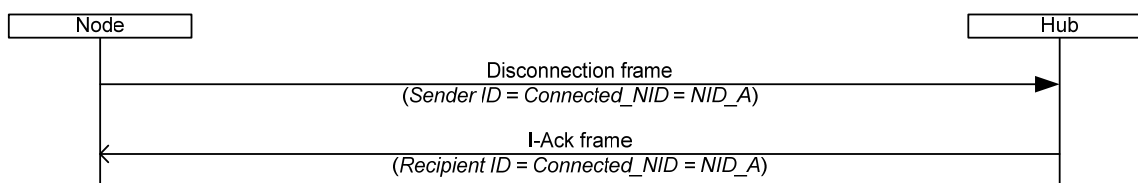
(a) Initiated by node
