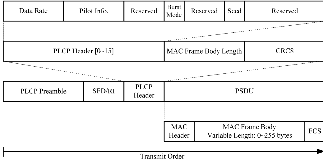
Figure 158 —HBC Packet Structure
