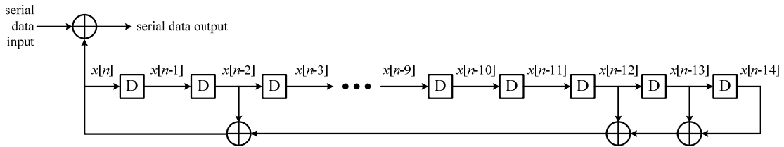
Figure 124 —Block diagram of a side-stream scrambler
