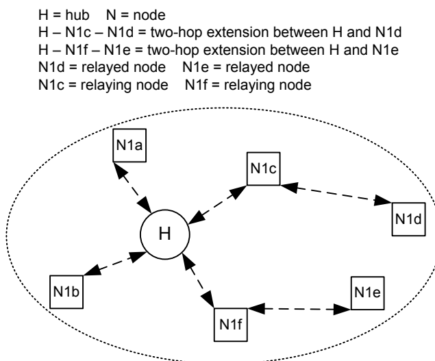
Figure 86—Two-hop extended star network topology
