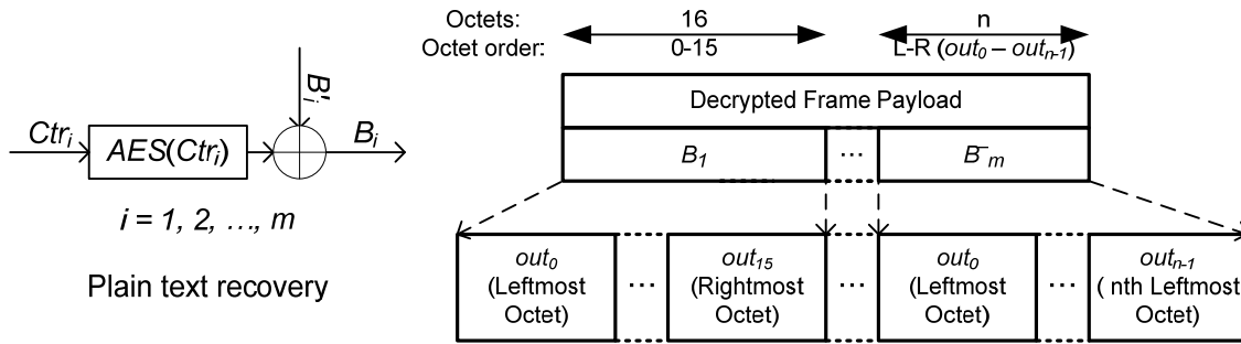
Figure 115 —Decrypted Frame Payload format for encrypted frames
