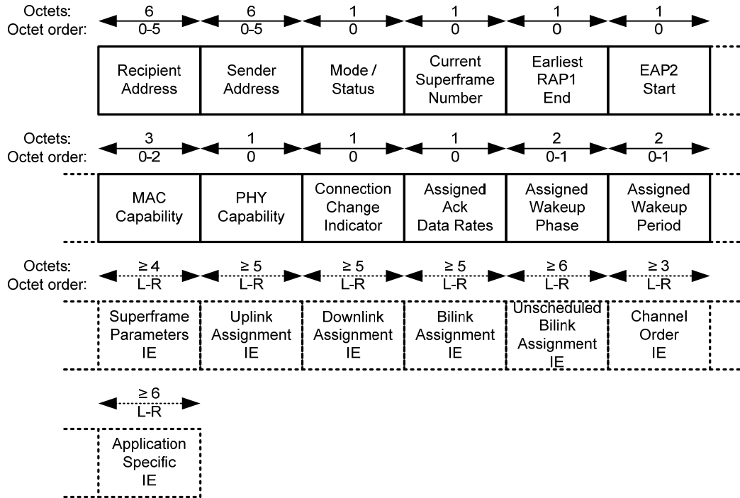
Figure 31—Frame Payload format for Connection Assignment frames
