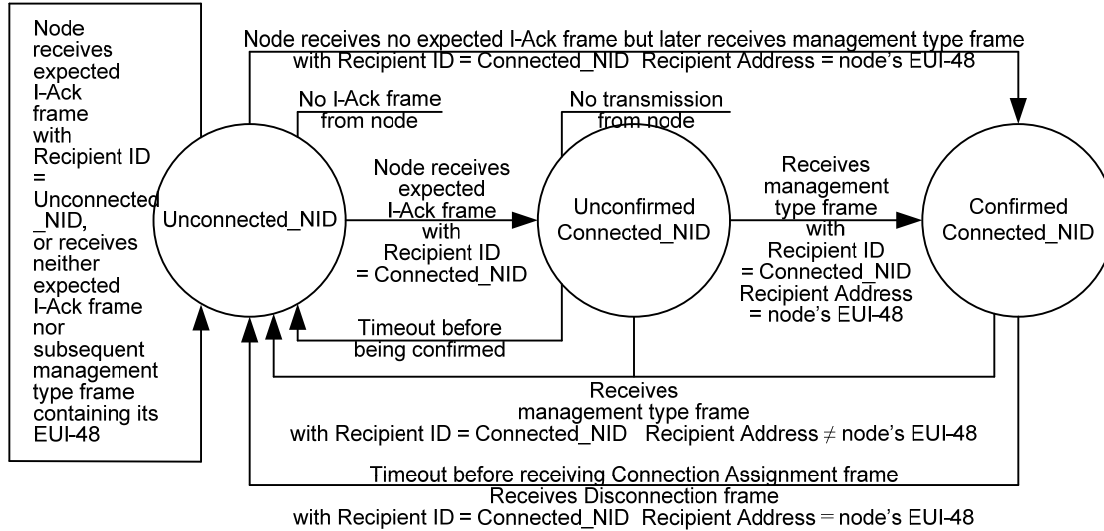
Figure 60—Node NID transition
