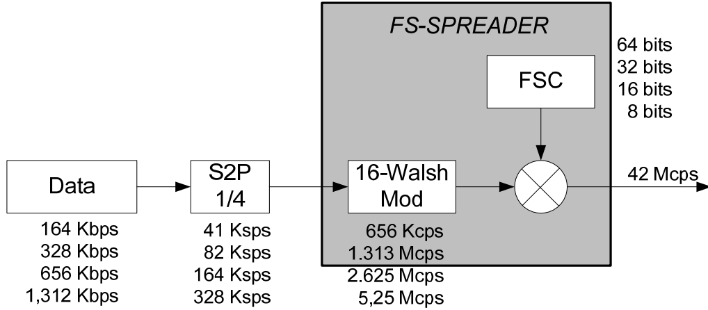
Figure 168 —S2P and FS-Spreader block diagram ( f_{CK} = 42 MHz)
