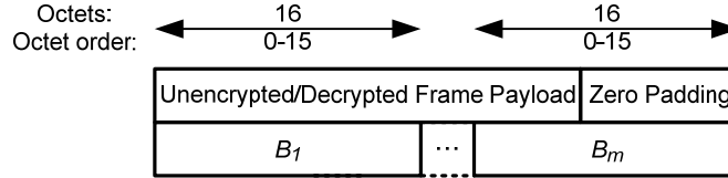
Figure 111 —Payload blocks B_1, \dots, B_m format
