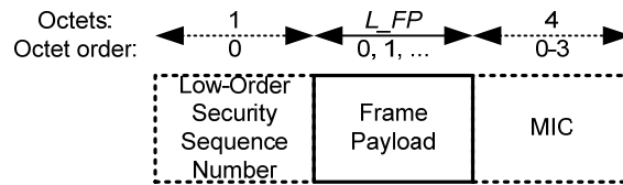
Figure 12—MAC Frame Body format
