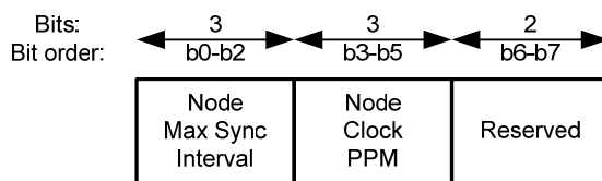
Figure 30—Max Sync Interval/Clock PPM format
