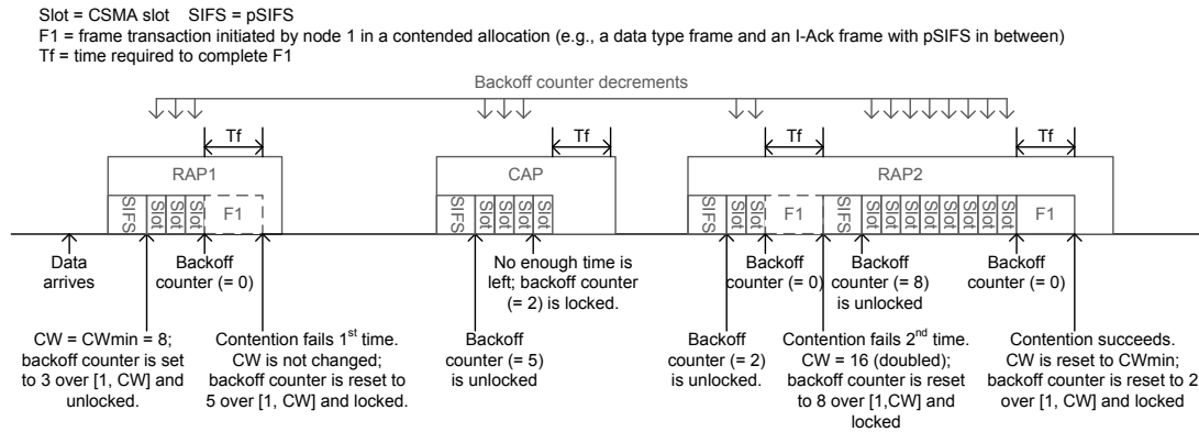
Figure 72—CSMA/CA Illustration
