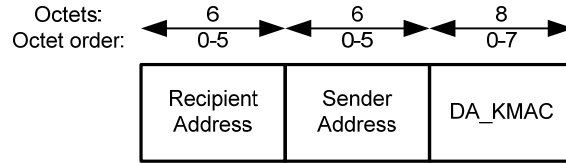
Figure 22—Frame Payload format for Security Disassociation frames
