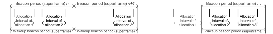
(a4) Round-robin allocations in beacon or non-beacon mode with superframes
