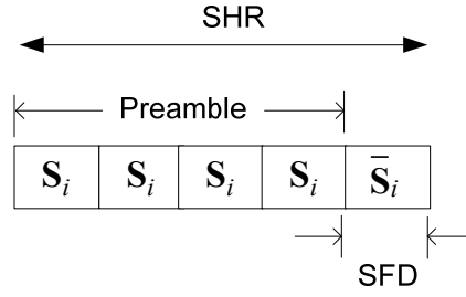
Figure 140 —Structure of SHR with OOK modulation
