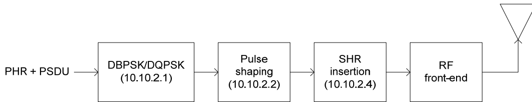
Figure 141 —Differentially encoded PSK modulation schematic diagram
