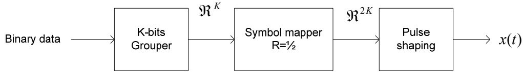
Figure C.1—On-off signaling as GPPM
