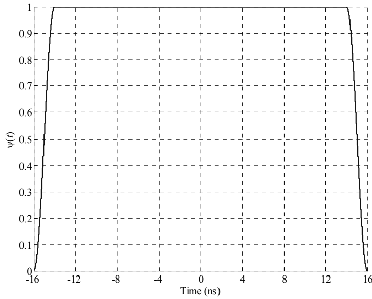
Figure 146 —Example of a window function for T_w = 32 ns and Tukey window T_u = T_d = 2 ns
