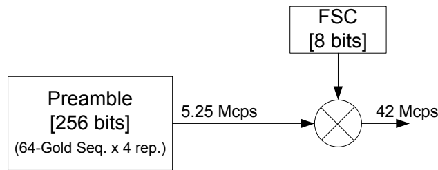
Figure 161 —Preamble generation block diagram ( f_{CK} = 42 MHz)
