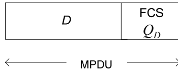
Figure 152 —MPDU with systematic bits for HARQ
