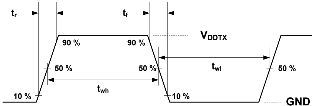
Figure 172 —Transmit timing information
