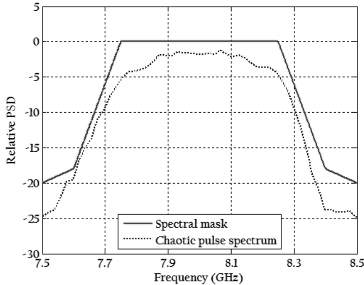
Figure 149 —Power spectral density of chaotic pulses with 10db bandwidth of 500 MHz
