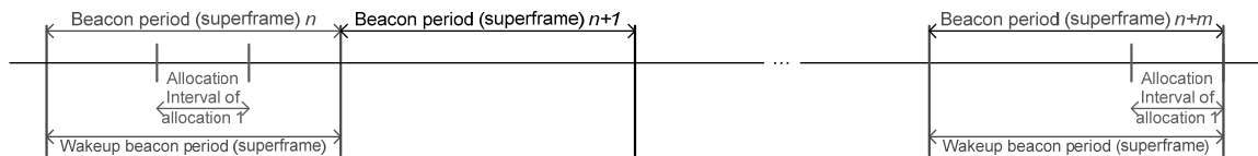
(b3) shifted and reduced/expanded m-periodic allocation in beacon or non-beacon mode with superframes
