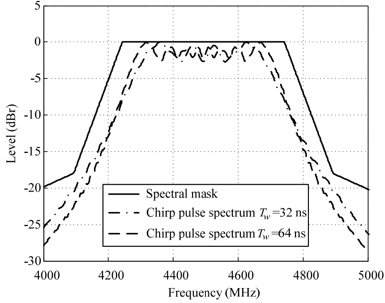
Figure 148 —PSD of chirp pulses centered at 4492.8 MHz fulfilling the transmit spectral mask
