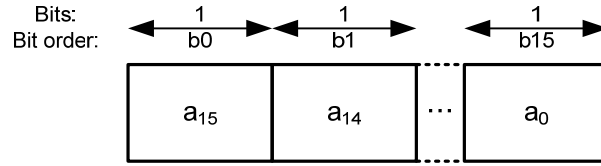
Figure 13—FCS format
