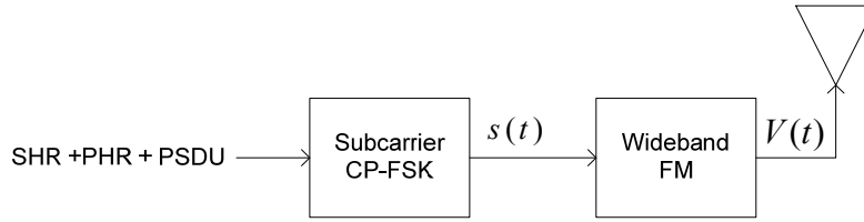
Figure 156 —FM-UWB transmitter block diagram
