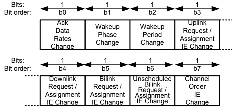
Figure 28—Connection Change Indicator format
