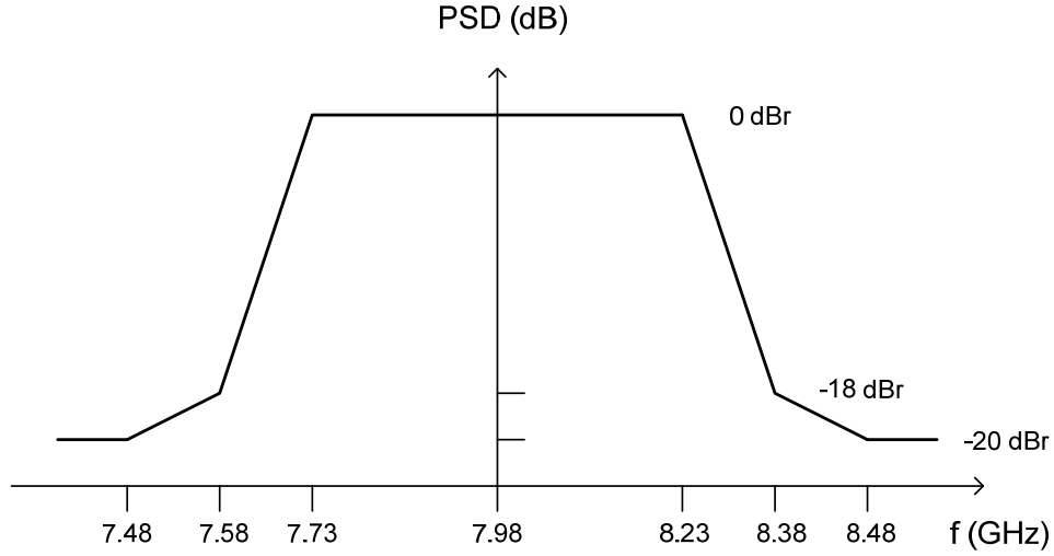
Figure 144 —Transmit spectral mask for band 7
