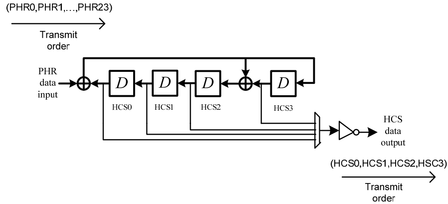
Figure 134 —CRC4-ITU data processing
