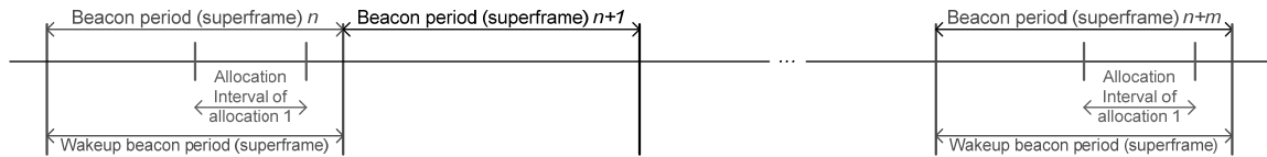
(b2) Shifted m-periodic allocation in beacon or non-beacon mode with superframes
