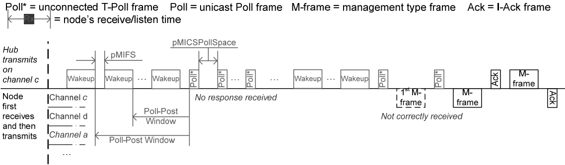
(a) Using Wakeup and T-Poll frames
