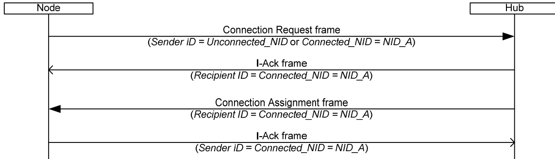
Figure 68—Connection procedure
