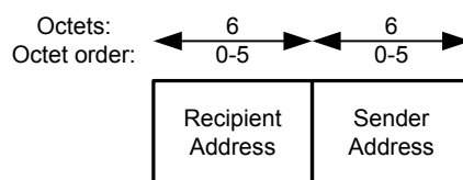
Figure 40—Frame Payload format for Wakeup frames
