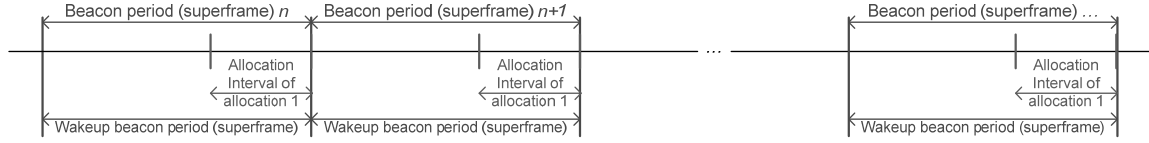
(a2) Shifted 1-periodic allocation in beacon or non-beacon mode with superframes
