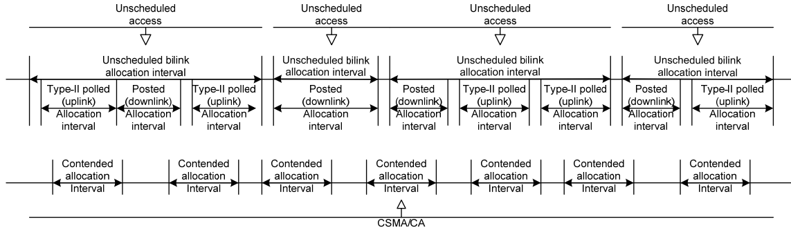
Figure 67—Allocation intervals and access methods permitted for non-beacon mode without superframes
