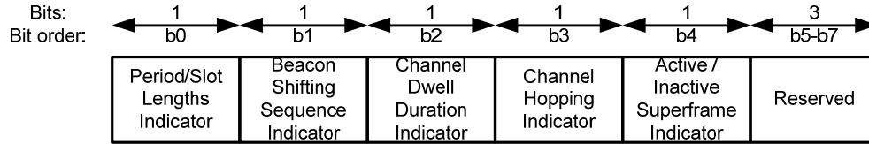
Figure 46—Superframe Parameters Bitmap format
