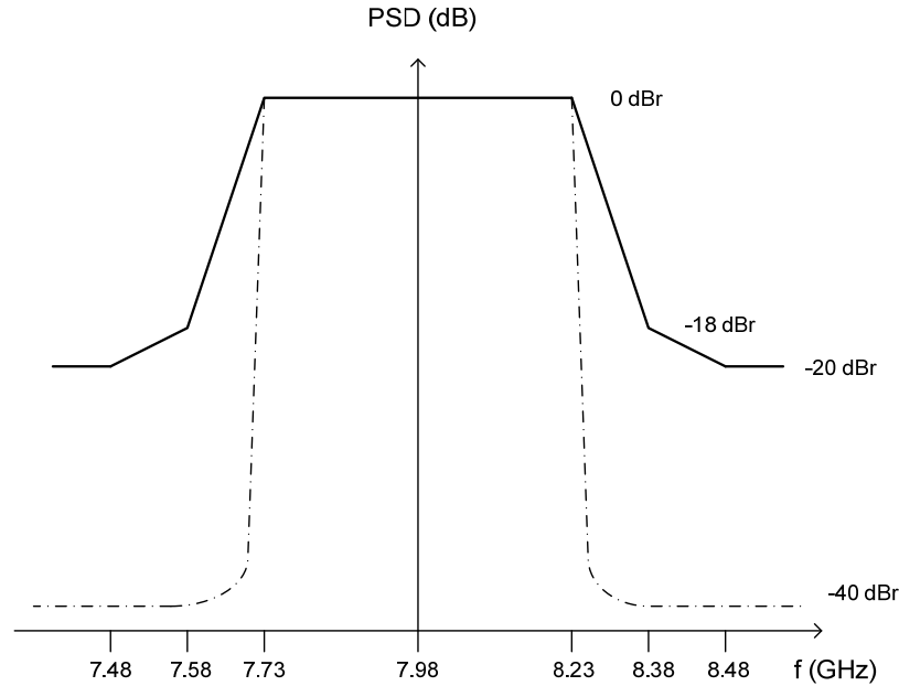
Figure 157 —Frequency spectrum of FM-UWB signal at 7.98 GHz center frequency
