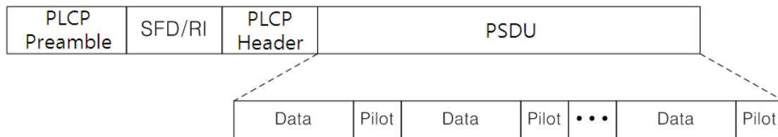
Figure 169 —Pilot Insertion in PSDU
