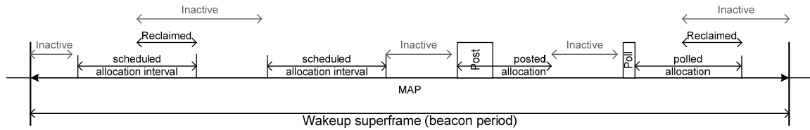
(b) Non-beacon mode without superframes
