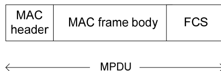
Figure 130 —MPDU structure
