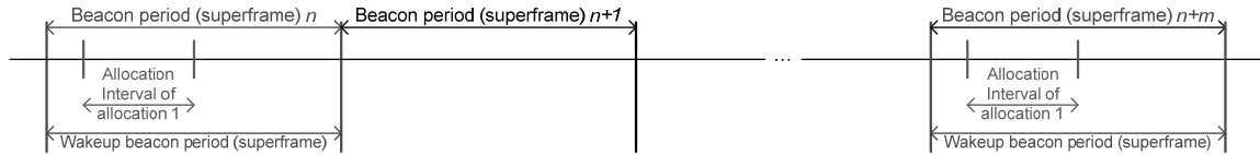
(b1) Assigned m-periodic allocation in beacon or non-beacon mode with superframes
