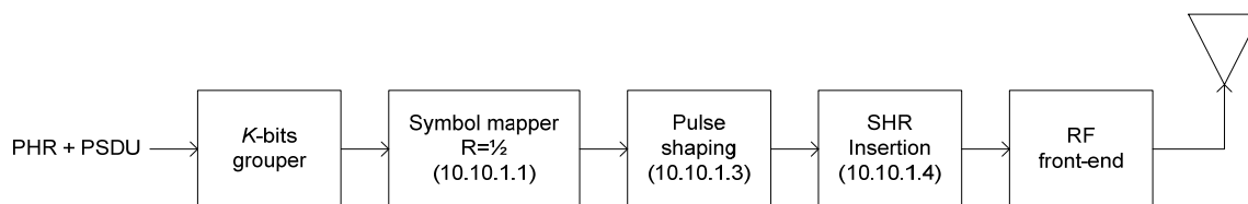
Figure 139 —On-off modulation schematic diagram
