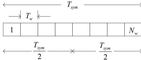
Figure 137 —UWB symbol structure
