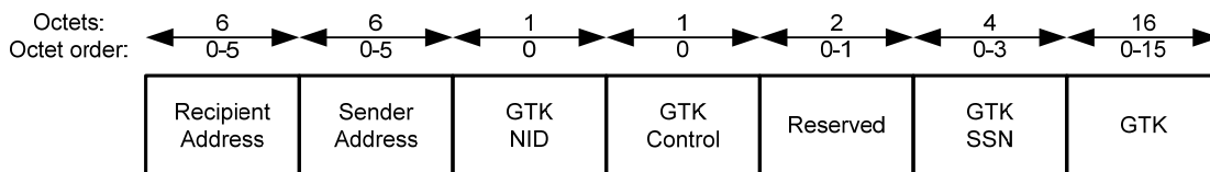
Figure 25—Frame Payload format for GTK frames
