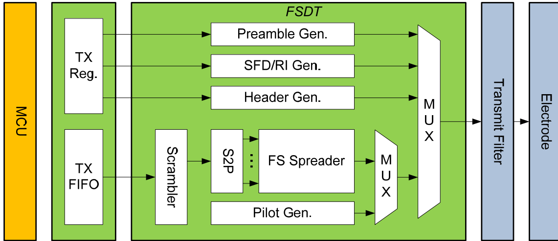
Figure 159 —Reference HBC transmitter block diagram
