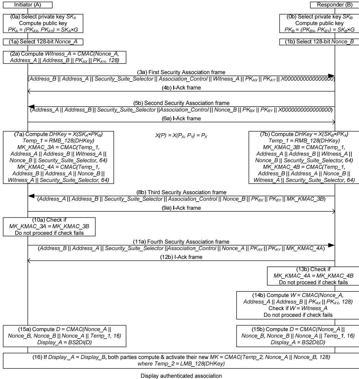
Figure 105 —Display authenticated association procedure
