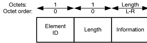
Figure 44—IE format—general
