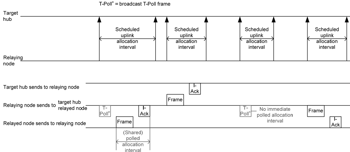
Figure 89—Scheduled uplink allocation for relaying node to send broadcast T-Polls and to relay frames
