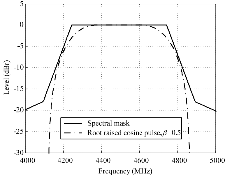
Figure 145 —PSD of r(t) centered at 4492.8 MHz satisfying the transmit spectral mask
