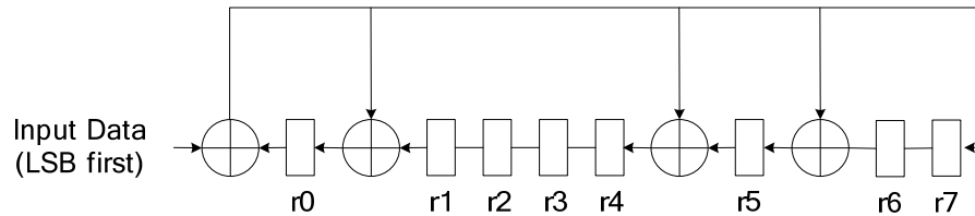
Figure 166—CRC8 implementation
