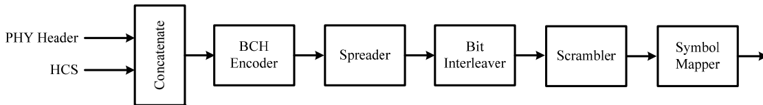
Figure 117 —Block diagram of PLCP header construction for transmission
