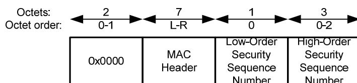
Figure 109 —Nonce format
