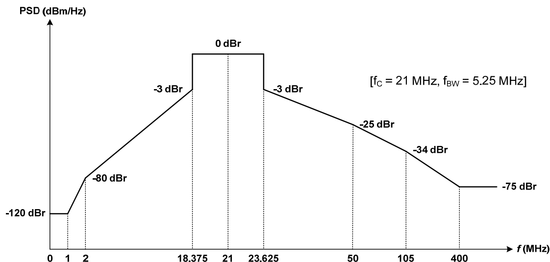
Figure 171 —Transmit spectral mask
