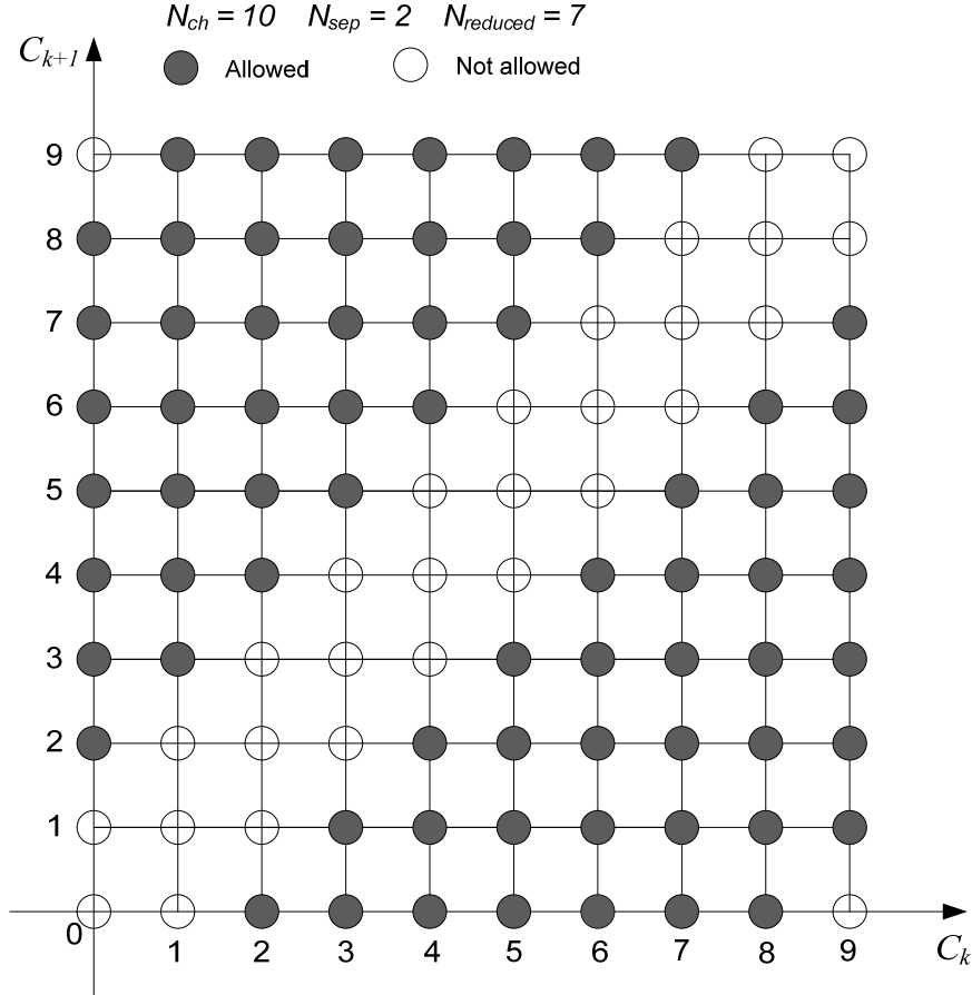
Figure 100 —Channel separation in consecutive hops
