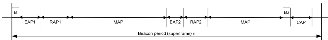
Figure 64—Layout of access phases in a beacon period (superframe) for beacon mode
