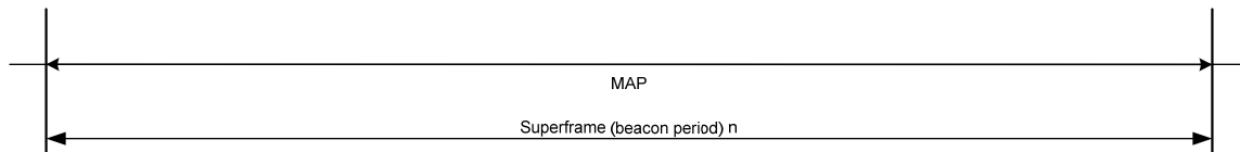
Figure 66—Layout of access phases in a superframe (beacon period) for non-beacon mode
