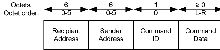
Figure 34—Frame Payload format for Command frames
