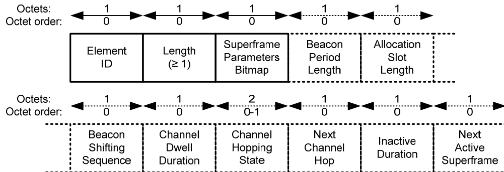
Figure 45—Superframe Parameters IE format
