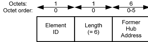
Figure 58—Former Hub Address IE format
