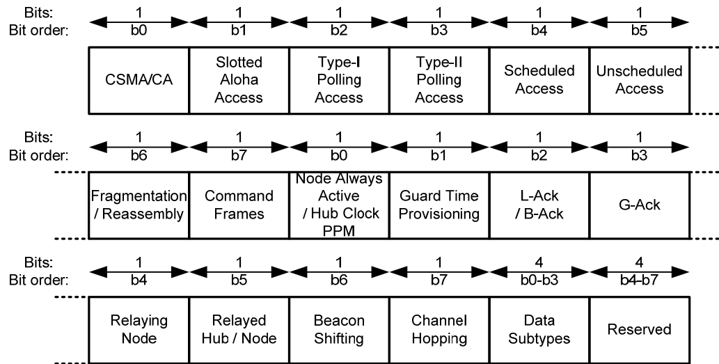
Figure 42—MAC Capability format
