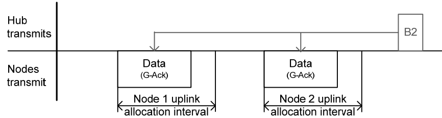
Figure 61—Group acknowledgement (G-Ack)
