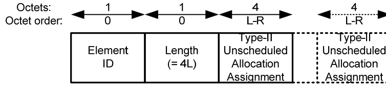
Figure 53—Type-II Unscheduled Bilink Assignment IE format
