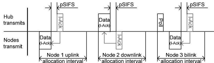
Figure 62—Immediate acknowledgement (I-Ack) illustration
