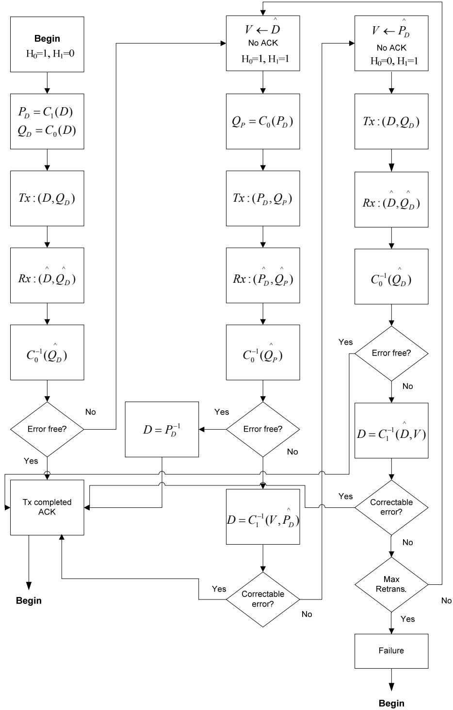
Figure 155 —Flow diagram of Type II HARQ
