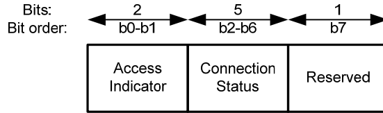
Figure 32—Mode/Status format
