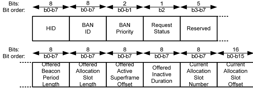
Figure 36—Command Data format for Command—Active Superframe Interleaving Response frames
