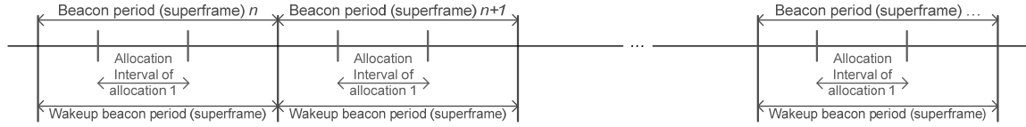
(a1) Assigned 1-periodic allocation in beacon or non-beacon mode with superframes
