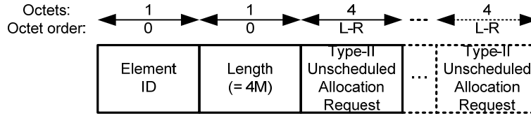
Figure 49—Type-II Unscheduled Bilink Request IE format
