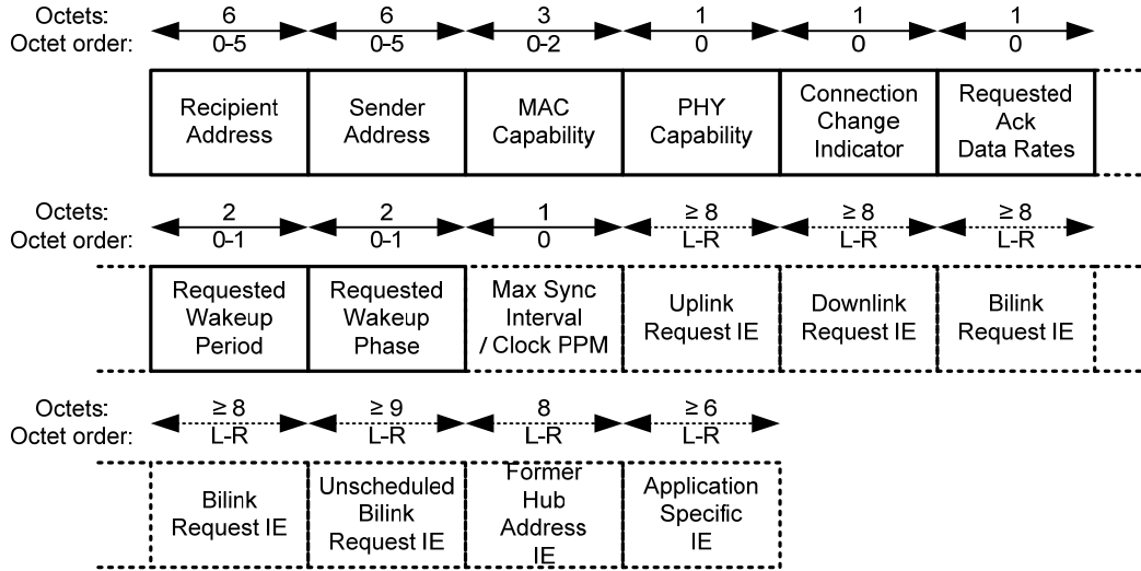
Figure 27—Frame Payload format for Connection Request frames
