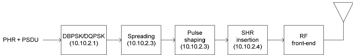
Figure 142 —Schematic diagram of DPSK modulation with spreading
