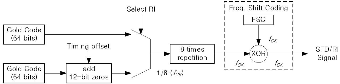
Figure 163 —SFD/RI signal generation block diagram ( f_{CK} = 42 MHz)
