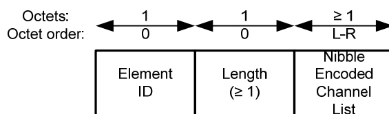
Figure 55—Nibble Encoded Channel Order IE format
