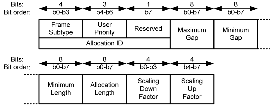
Figure 48—Allocation Request format
