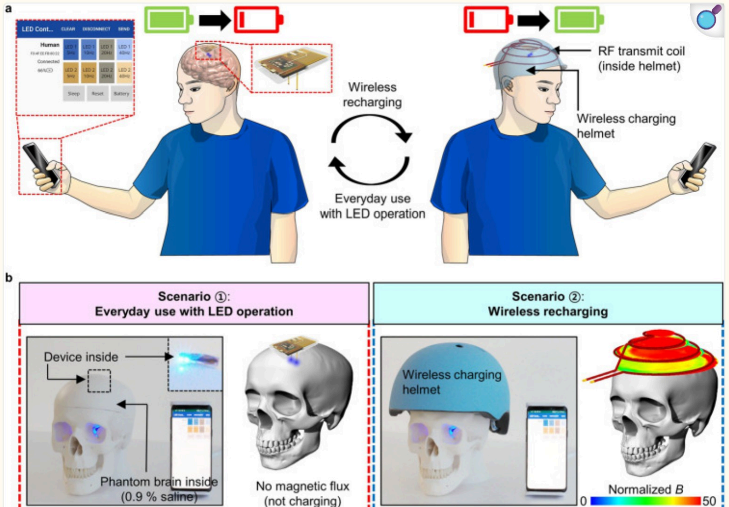
Fig. 5. Proof-of-concept demonstration of fully implantable, wireless rechargeable optoelectronic systems for potential operation in a human brain.
