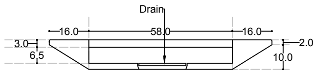
Section
