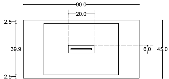
Top plan
