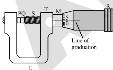
Positive zero error (2 division error) i.e., + 0.002 cm
