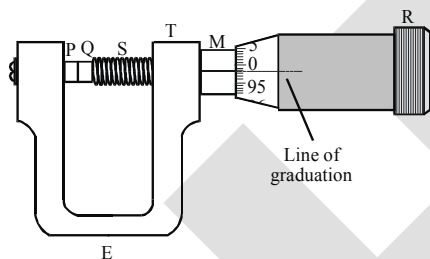
Negative zero error (3 division error) i.e., - 0.003 cm
